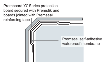
External corner
