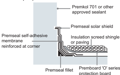
Concrete parapet
