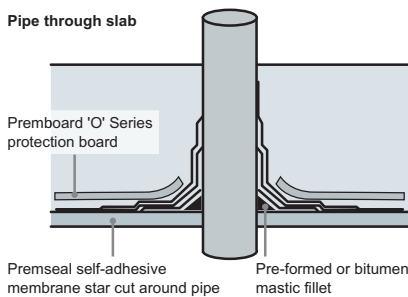
Pipe through slab
