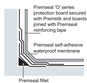
Internal corner
